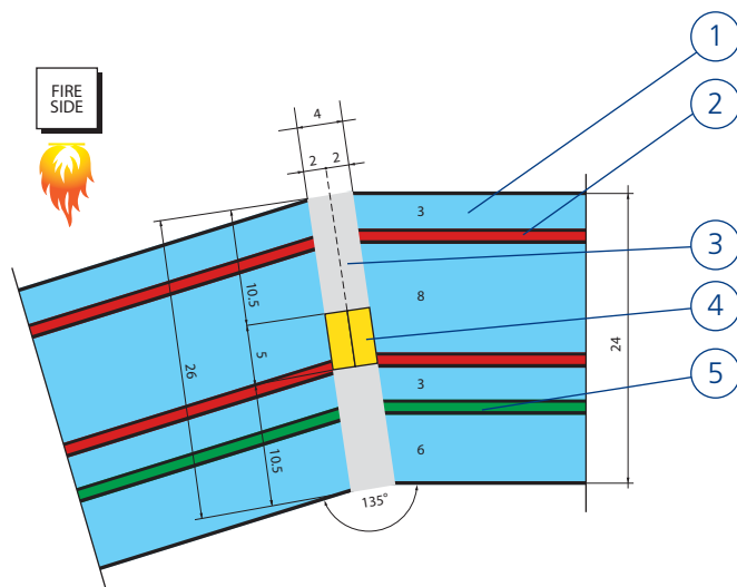
Steel frame (in mm)
