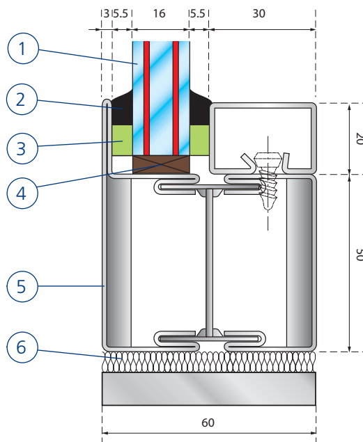
Steel frame (in mm)
