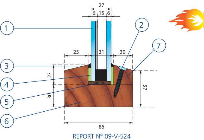
Timber frame (in mm)
