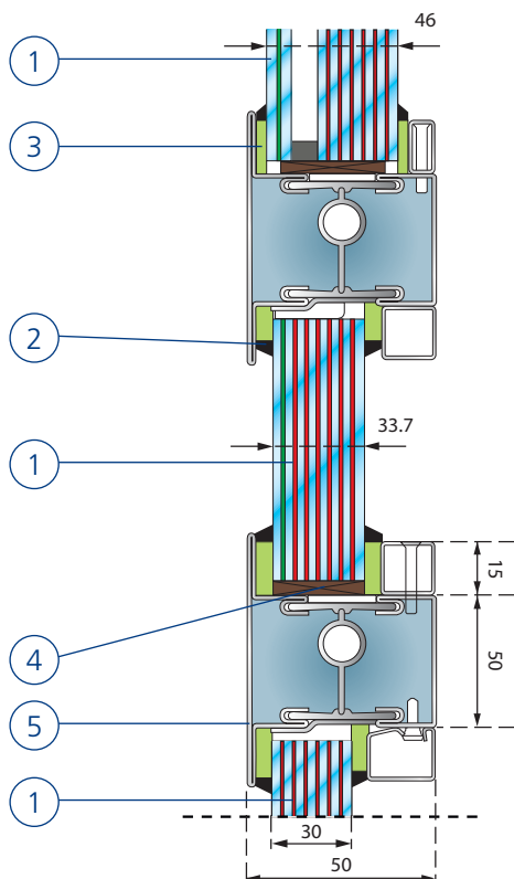
Steel frame (in mm)
