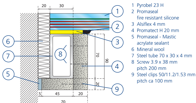
Steel frame EI 45* (in mm)
