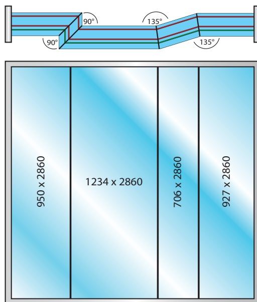
Example of assembly (in mm) Unlimited partition
