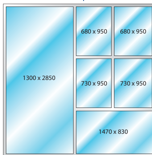
Example of assembly (in mm) Unlimited partition
