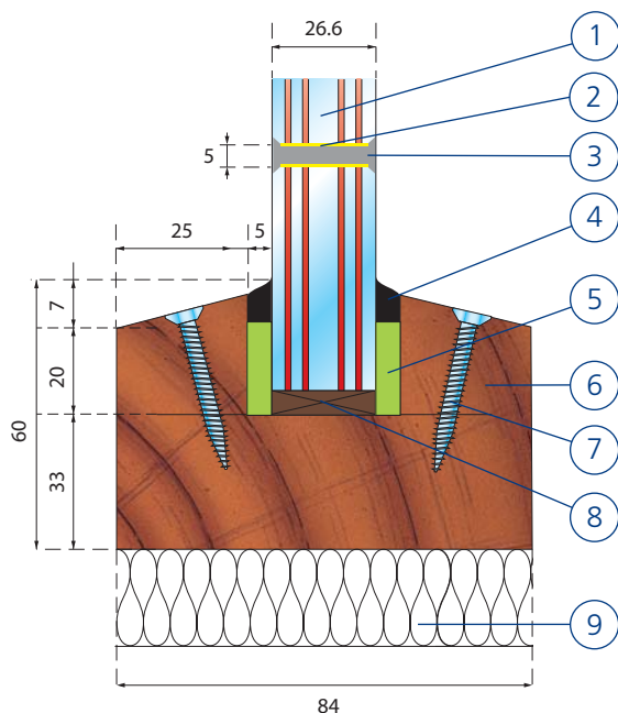
Timber frame (in mm)
