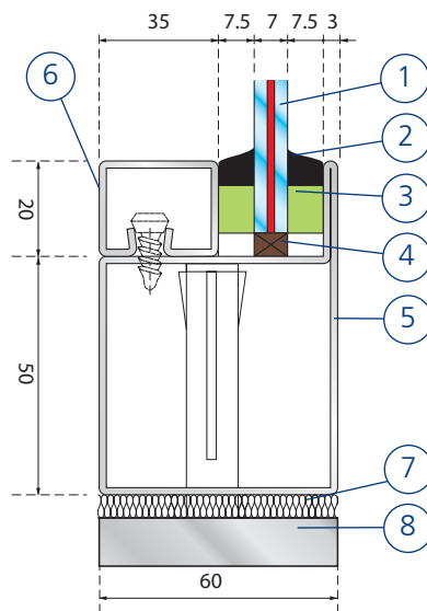
Steel frame (in mm)
