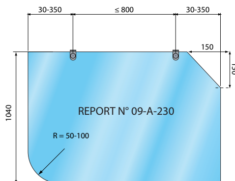
Example of installation (in mm)
