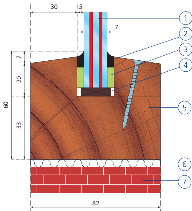
Timber frame (in mm)
