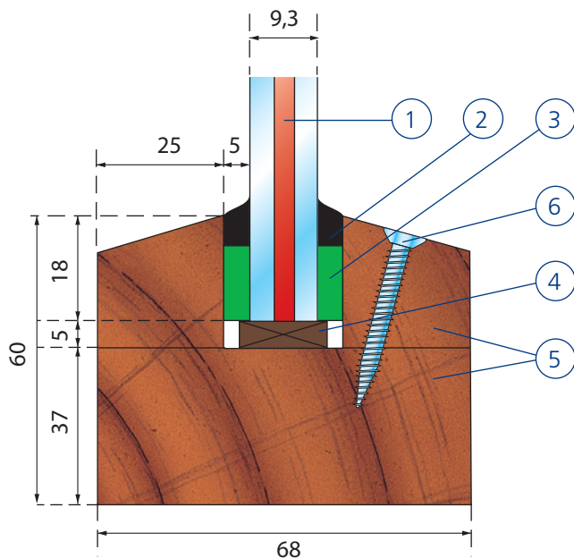
Timber frame (in mm)
