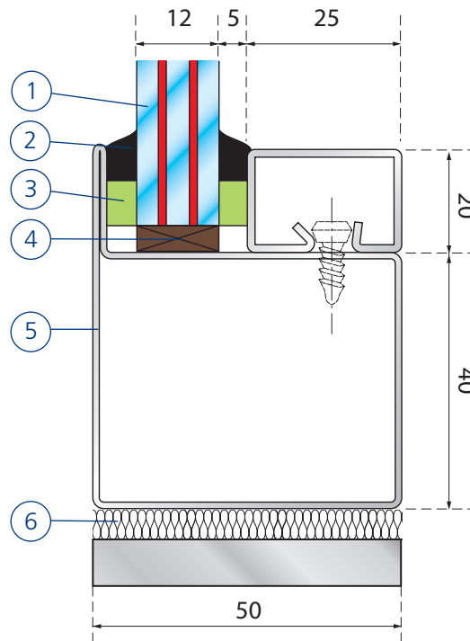
Steel frame (in mm)
